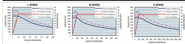
EDF-160 mm BORE WITH FANUC 30/37 kW MOTOR
