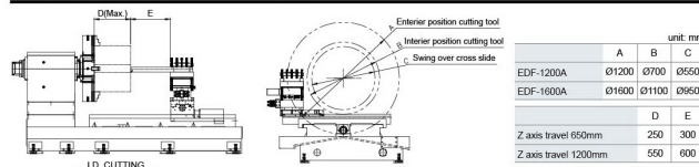
PROCESSING CAPACITY FOR 6-WAY TURRET
