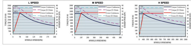
PROCESSING CAPACITY FOR 4-WAY TURRET
